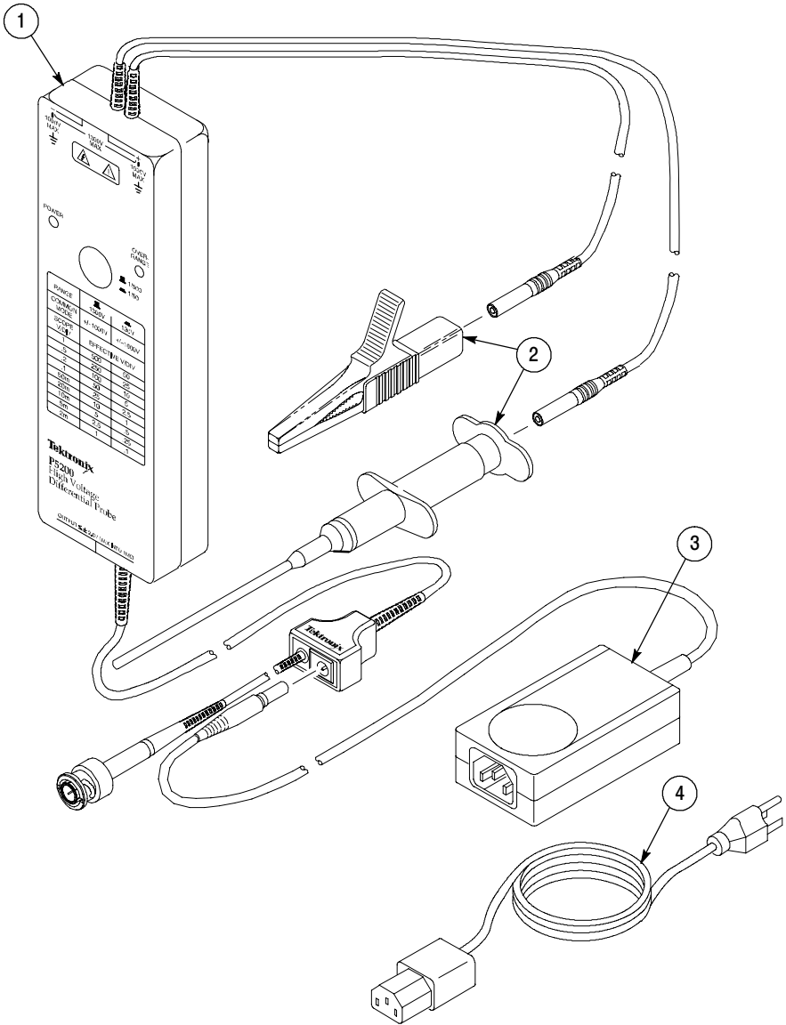
Figure 9: P5200 High Voltage Differential Probe and replaceable accessories
