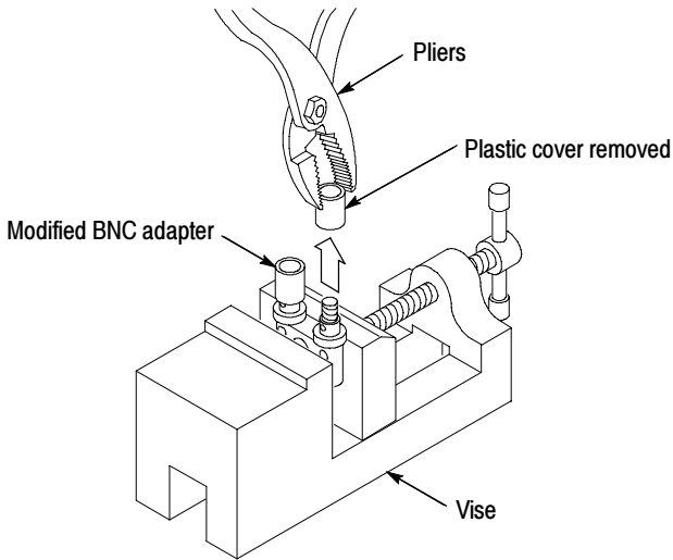
Figure 7: Removing plastic covers from binding posts
