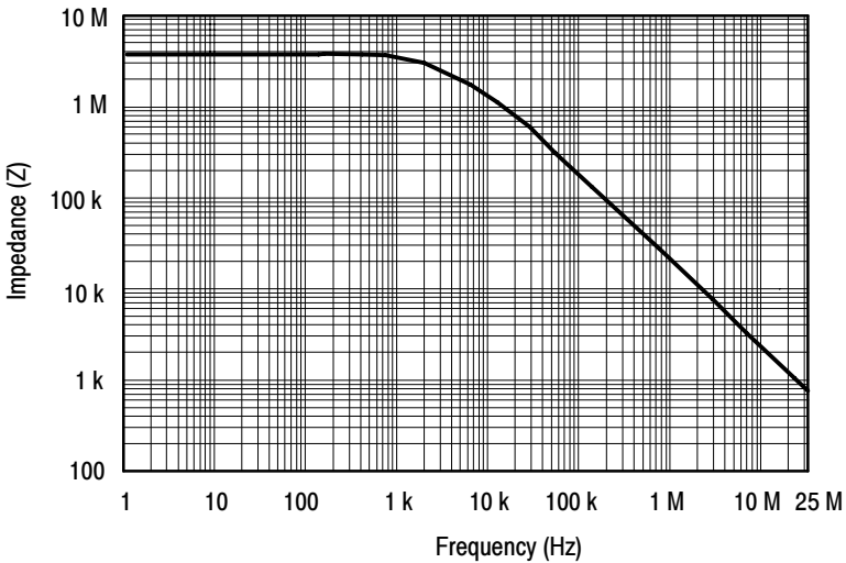
Figure 3: Input impedance vs. frequency
